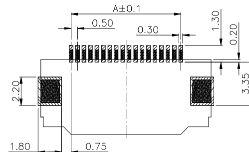
(Tolerance:0.05) Recommended PCB Layout
