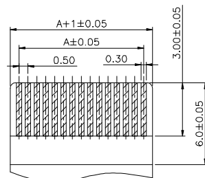
FFC/FPC Dimension(Thickness 0.30 mm)
