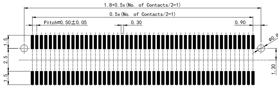
PCB Layout For Surface Mounting
