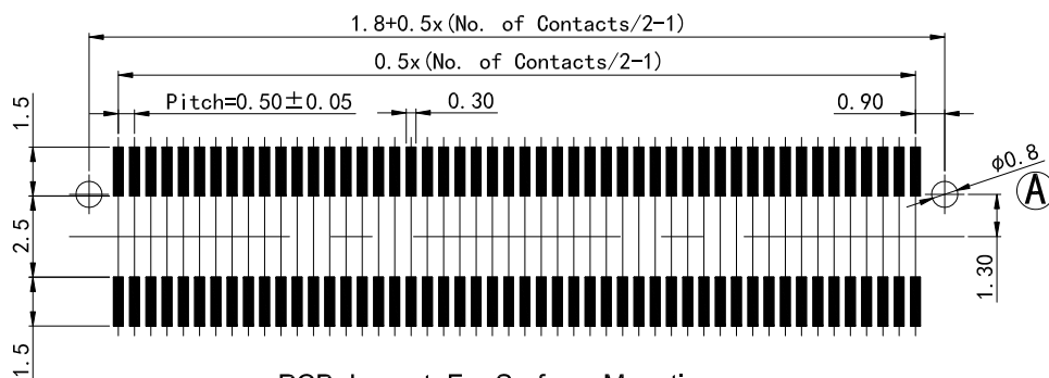
PCB Layout For Surface Mounting
