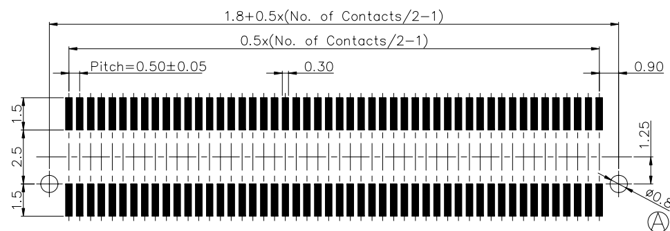
PCB Layout For Surface Mounting
