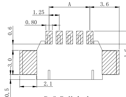
P. C. B Hole Layout
