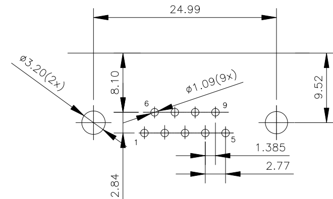
P.C.B. LAYOUT(TOLERANCE:±0.05)TOP VIEW
