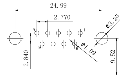
P.C.B. LAYOUT (TOLERANCE: ±0.05) TOP VIEW
