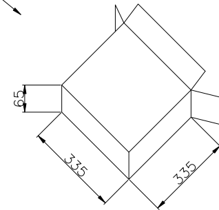
內箱 (2000pcs/盒)
