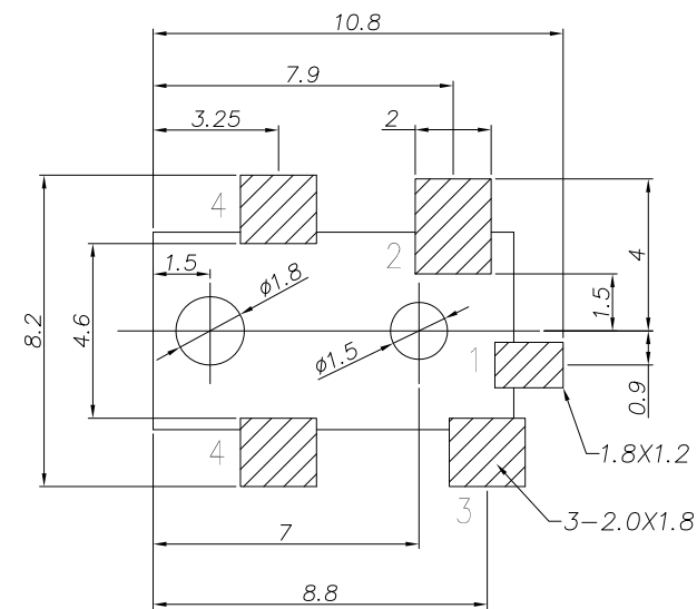
Recommended PCB Layout (Tolerance±0.05) (Copper-sided View)
