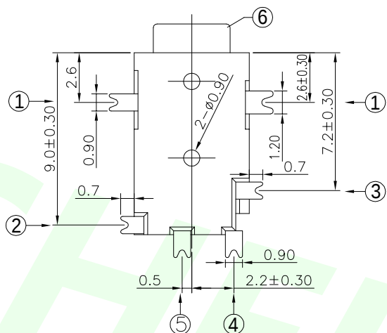
SCHEMATIC
